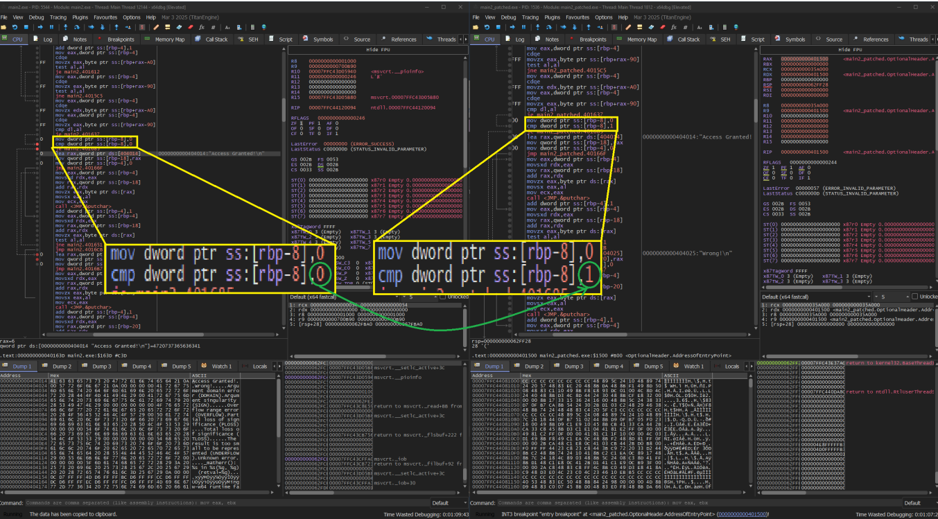
x64dbg - An open-source x64/x32 debugger for windows.
