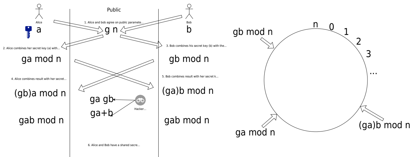
Diffie-Hellman key exchange
